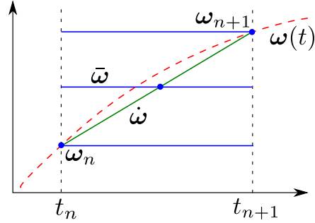
Figure 13: Angular velocity approximations for the integral: Red: true velocity. Blue: zeroth order approximations (bottom to top: forward, midway and backward). Green: first order approximation.
