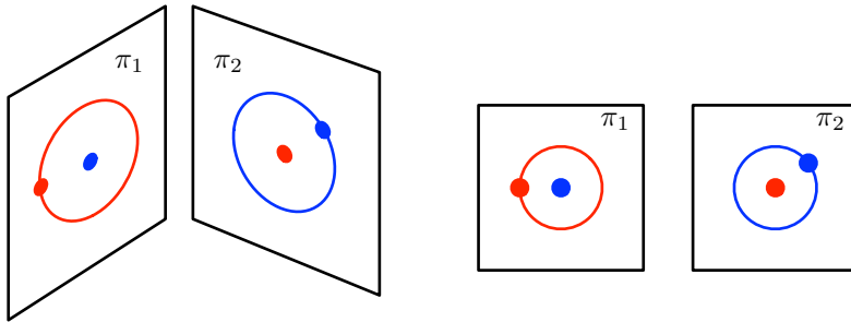
Figure 9: Rotations in \mathbb{R}^4 . Two orthogonal rotations are possible, on two orthogonal planes \pi_1 and \pi_2 . Rotations of a vector \mathbf{x} (not drawn) in the plane \pi_1 cause the two components of the vector parallel to this plane (red dot on \pi_1 ) to describe a circumference (red circle), leaving the other two components in \pi_2 unchanged (the red dot). Conversely, rotations in the plane \pi_2 (blue dot on blue circle in \pi_2 ) leave the components in \pi_1 unchanged (blue dot). The sketch on the right better illustrates the situation by resigning to draw unrepresentable perspectives in \mathbb{R}^4 , which might be misleading.
